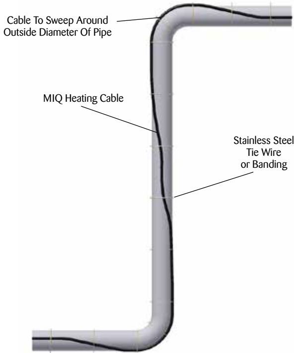
Illustration C: Pipe Elbow . . .
