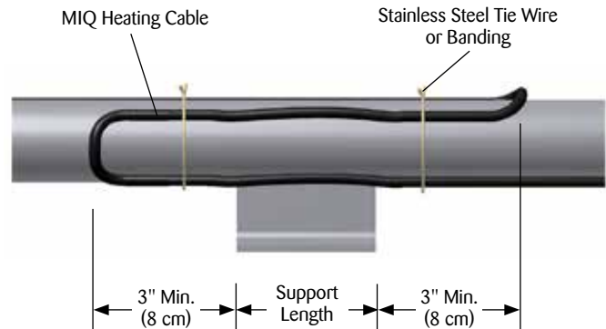
Illustration D: Pipe Support . . .
