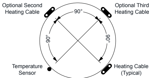
Heating Cable vs. Sensor Location (Line Sensing Control)
